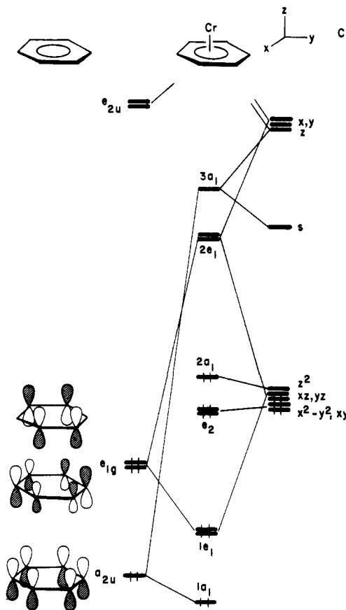
Figure 2. Construction of the valence orbitals in benzene-Cr. 14 summarized in Tables IV-VII, respectively.
