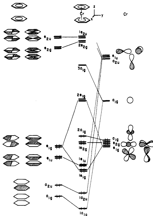
Figure 1. A generalized molecular orbital diagram for bis(benzene)metal complexes of D_{6h} symmetry following the analysis of (C_6H_6)_2Cr by: Shustorovich, E.; Dyatkina, M. E. Dokl. Akad. Nauk. SSSR 1959, 128, 1234. Photoelectron spectroscopic studies of gaseous bis(benzene), bis(toluene), and bis(mesitylene) complexes of Cr, Mo, and W agree in assigning the lowest ionization energy to ionization from 2a_{1g} . This ionization energy from the ^2A_1 ground state is 5.4–5.5, 5.2–5.3, and 5.0–5.2 eV for the benzene, toluene, and mesitylene complexes, respectively. Generally, the chromium and molybdenum complexes have the lowest and highest ionization energy, respectively, for a given arene ligand set. The next band has been assigned to the ^2E_{2g} ion state and the next two (unresolved for chromium) successively to the ^2E_{1u} and ^2E_{1g} ion states. For a general discussion of photoelectron studies of (arene)metal complex, see: Green, J. C. Struct. Bonding , 1981, 43, 37.
